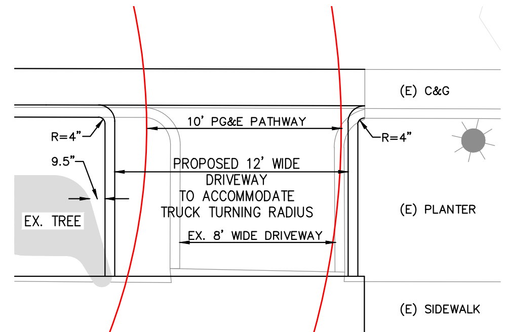
PROPOSED NORTH DRIVEWAY 1"=5'
